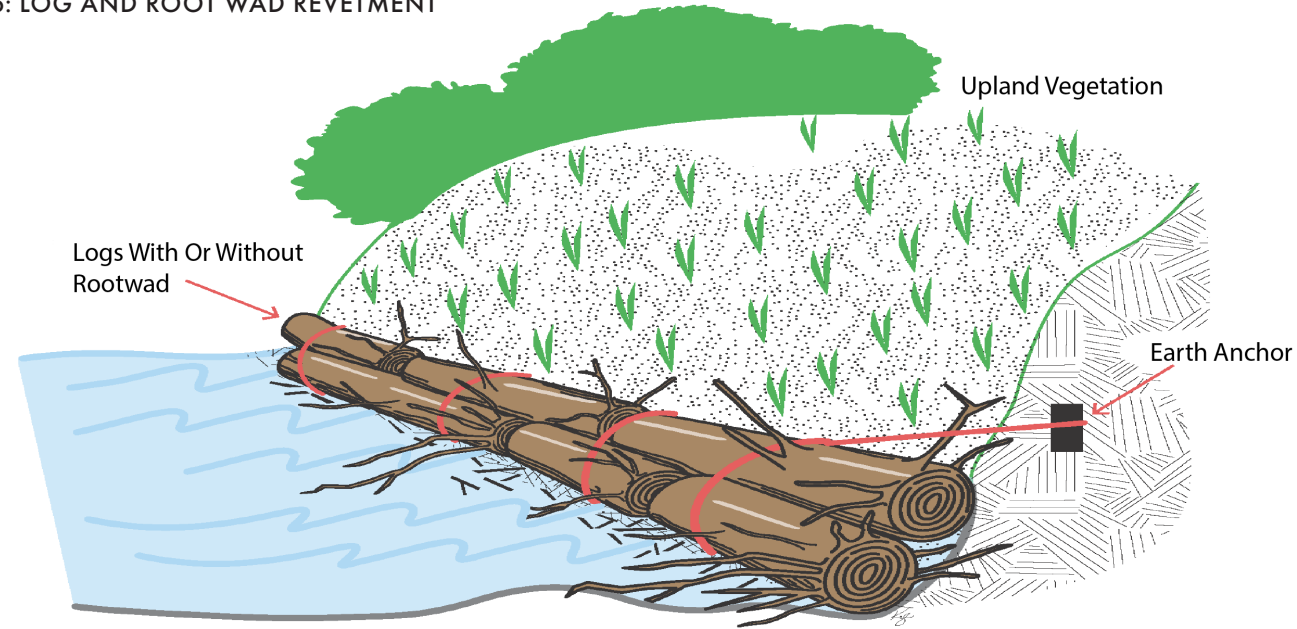
Level 3 FIGURE 6: LOG AND ROOT WAD REVETMENT
